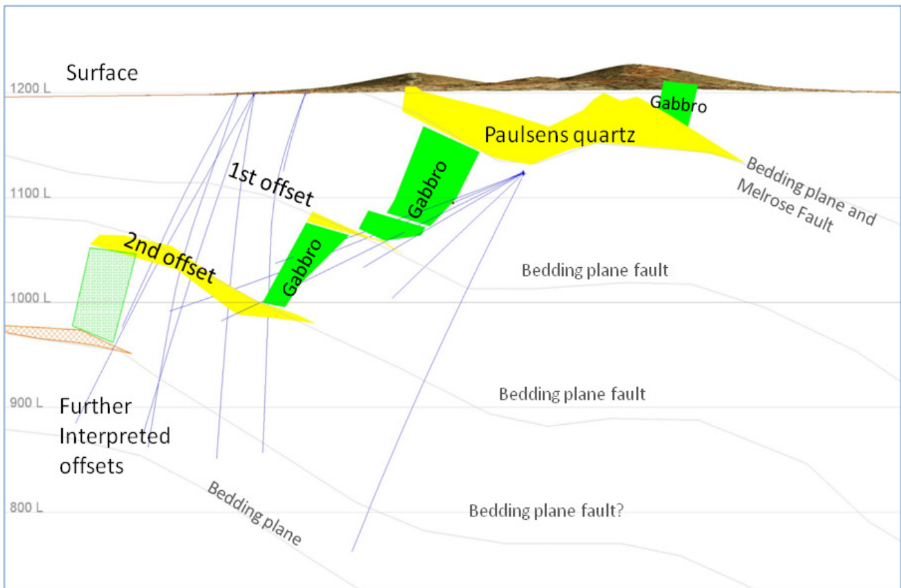
FIG 1 - CROSS SECTION OF INTREPRETATION OF QUARTZ LODES AND GABBRO OFFSET POSITION
