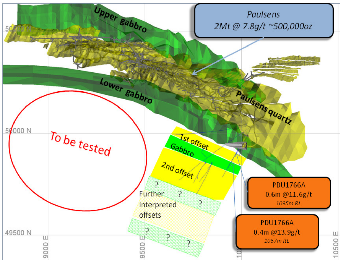
FIG 2 - PLAN VIEW OF INTREPRETATION OF QUARTZ LODS AND GABBRO OFFSET POSITION
