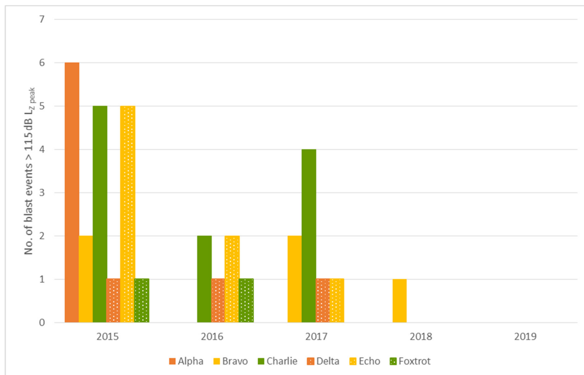
Figure 5-13: Airblast monitoring - number of blast events where airblast levels > 115 dB L_{Z\ peak} were recorded
