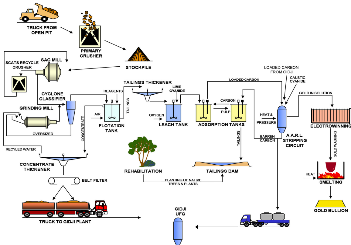
Figure 2-2: Gold ore treatment flowchart
