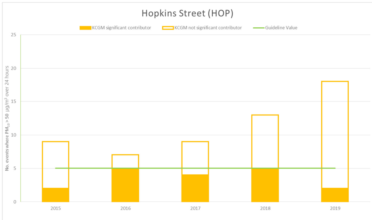
Figure 5-20: Hopkins Street (HOP) – number of days where 24-hour average PM 10 concentrations of greater than 50 µg/m 3 was recorded
