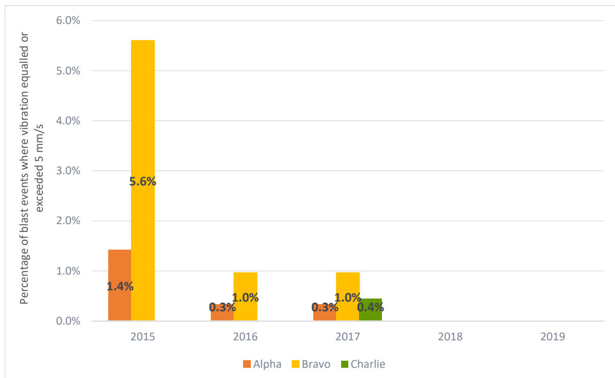
Figure 5-14: Vibration monitoring – frequency of blast events where vibration levels of > 5 mm/s were recorded
