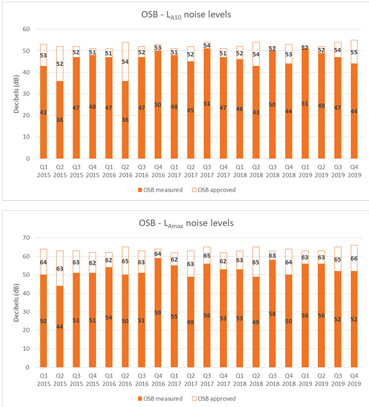
Figure 5-5: Outram Street Boulder (OSB) – compliance noise monitoring – L_{A10} and L_{Amax} noise levels
