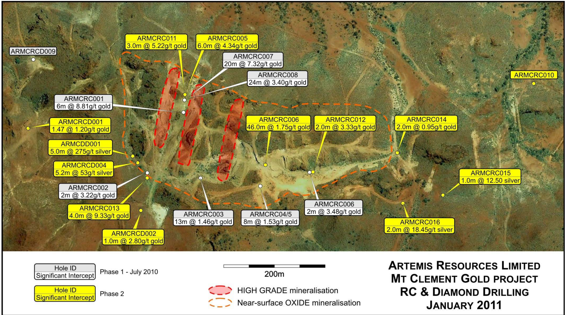
Figure 2: Image showing the location of drill holes and results - Mt Clement – January 2011
